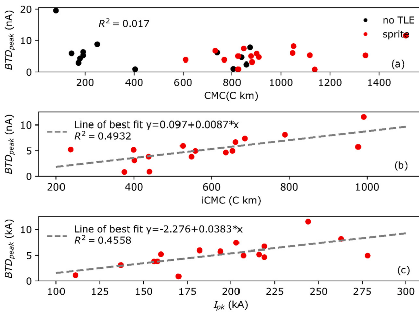
Fig. 9. (a) Independent ELF measurements of lightning return strokes associated with coincident BTDPeak current spikes show a wide range of possible CMC values, often below the threshold for sprite/halo initiation, and suggest that their peak amplitudes do not depend on the total amount of charge transferred. On the other hand, the probability of detecting a similar signature associated with a sprite-producing stroke increases for larger impulse charge moment changes (iCMC) (b) and peak currents (c).
