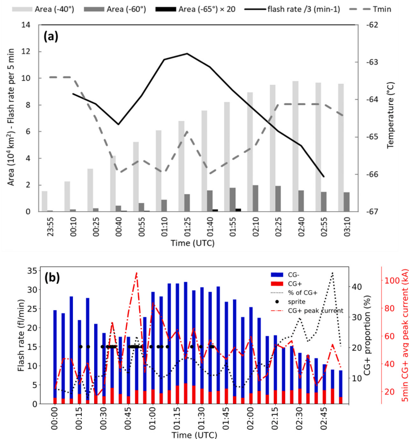
Fig. 2. Analysis of the storm structure and lightning activity, starting from about 15 min before the first sprite occurred. (a): Time series of minimum value of cloud top temperature T_{\min} and areas with CTT < -40^{\circ}\text{C} , < -60^{\circ}\text{C} and < -65^{\circ}\text{C} . The scale for areas is 10^4 \text{ km}^2 and A(-65) values are multiplied by 20. Solid black line shows the flash rate evolution for the same period. (b): CG flash rate by polarity (blue stacked bar for -CG, red stacked bar for +CG), +CG proportion (black dotted line) and 5-min average peak current of +CG (red dashed line). The black circles correspond to the time of observed sprites.
